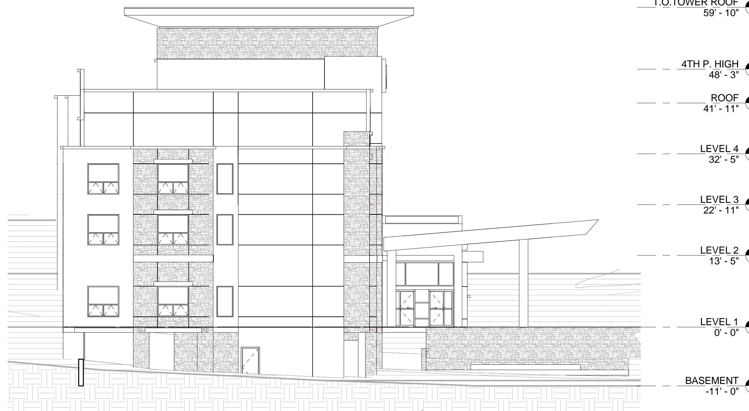
SOUTH ELEVATION
