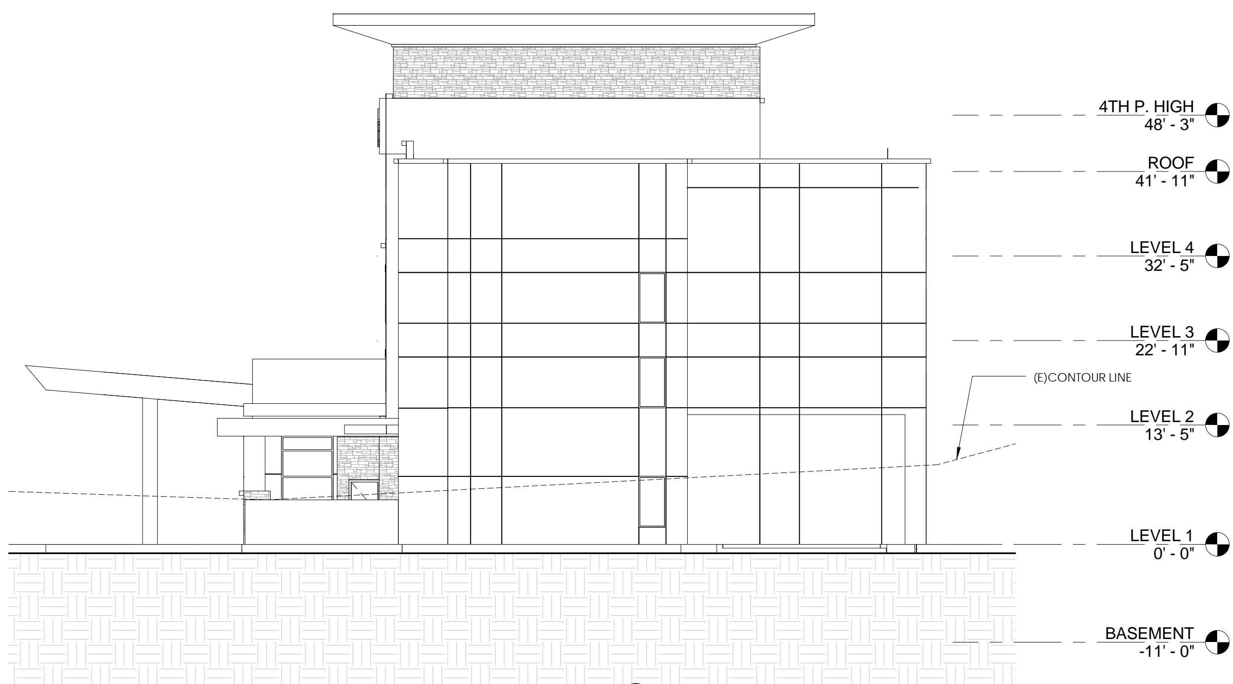
NORTH ELEVATION
